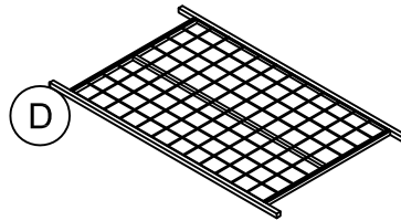
Base Frame T943600 X 3
